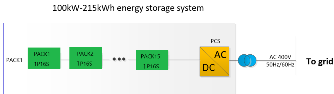
Figure 3-1 System Topology Diagram
